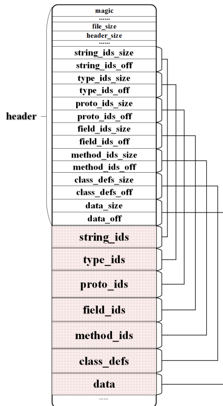
FIGURE 3.3 – DEX file format
