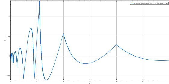
FIGURE 4.22 – Fast log error
