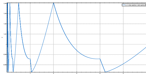
FIGURE 4.23 – Fast sqrt error
